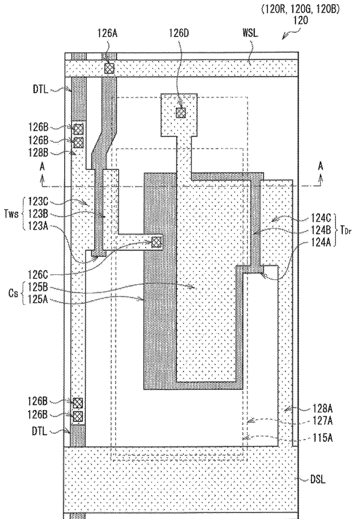
FIG. 17 PRIOR ART
