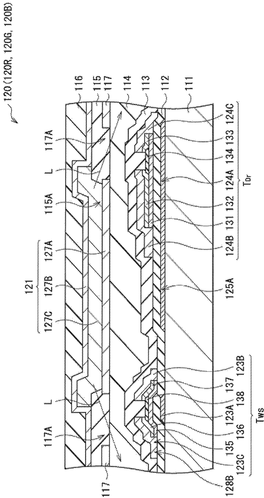
FIG. 18 PRIOR ART
